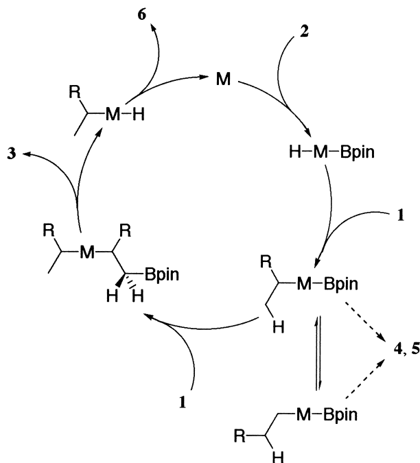
Fig. 1. Proposed catalytic cycle for dehydrogenative borylation ( M = \text{Rh}, \text{Ru} ).
